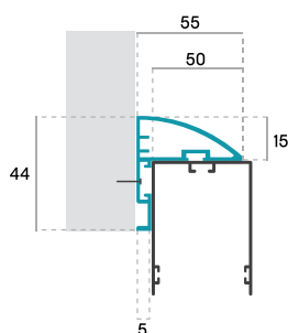
Front Fix standard
